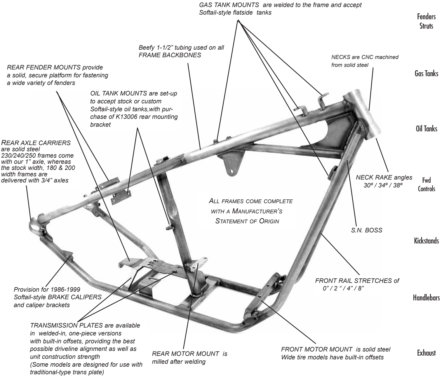
Frame shown is 4" stretch model
